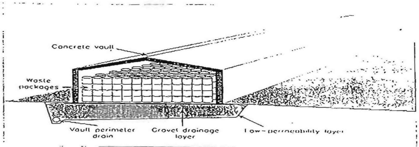
Figure C-2: Above-Ground Vault Disposal Facility 62
