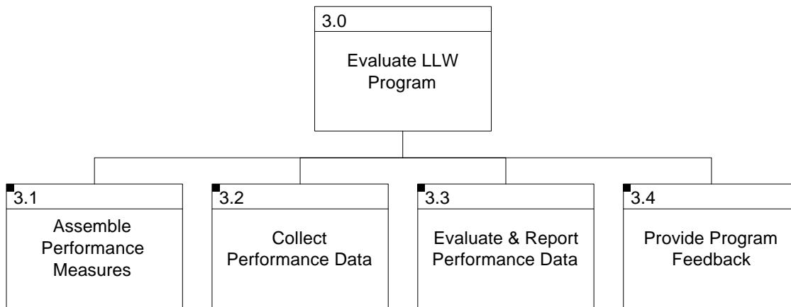
Figure 4.4: Evaluate Functions
