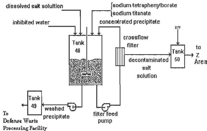
Figure 1. Process Flow Diagram of the In-Tank Precipitation Process
