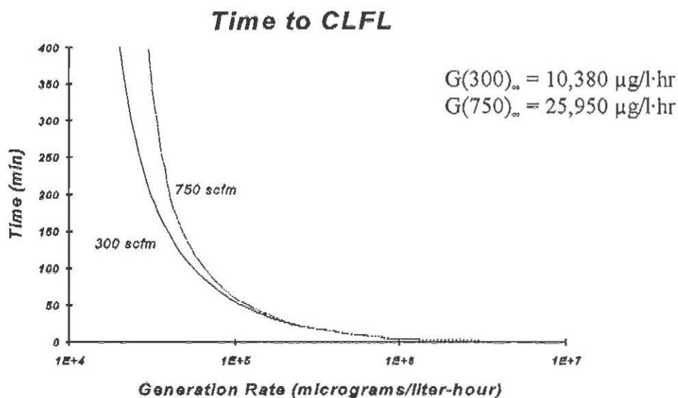
Figure 4. Calculated Time to CLFL
