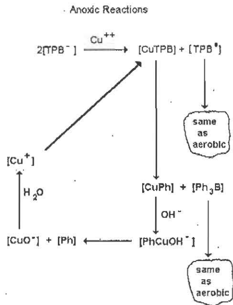
Figure A-2. Anoxic Decomposition Reaction Scheme
