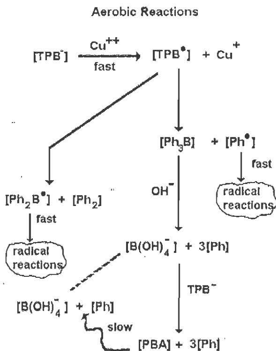
Figure A-1. Aerobic Decomposition Reaction Scheme
