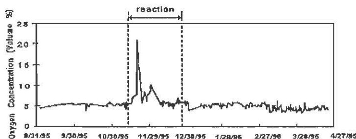
Figure 3. Tank 48H Oxygen History
