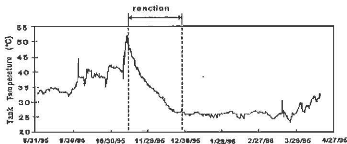
Figure 2. Tank 48H Temperature History
